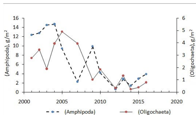
Fig. 1. Biomass dynamics of the main macrozoobenthos groups in the Petrozavodsk Bay of Onego Lake (2001–2016).
