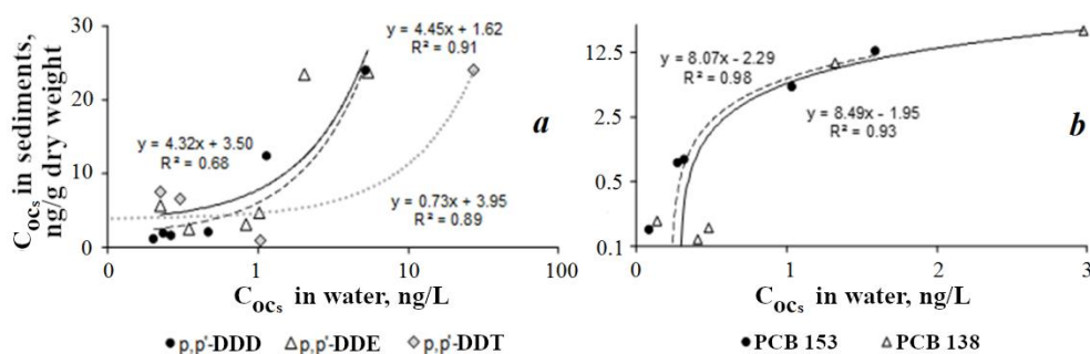
Fig. 3. Ratios of the DDT and its metabolites (a) and PCBs 153 and 138 (b) concentrations in the Salgir River sediments at st.1–6 by the respective values in water
