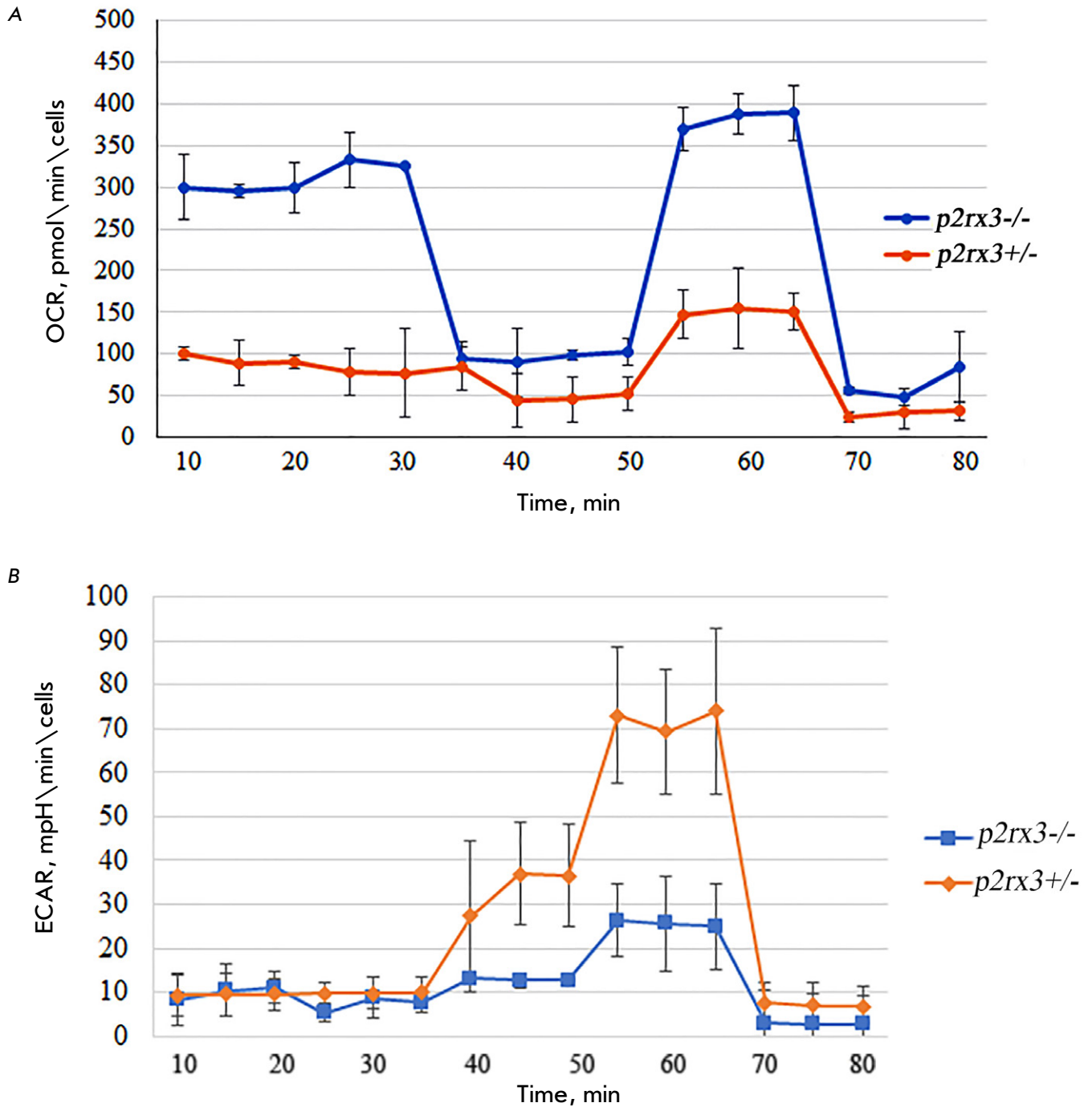
Fig. S1. Curves of the oxygen consumption rate during the mitostress test (A) and the rate of extracellular acidification during the glycotest (B) recorded using a Seahorse analyzer in real time
