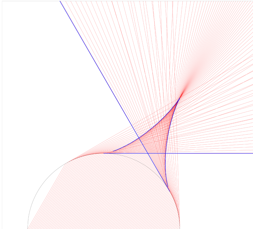
Fig. 5. Dielectric ball caustics for case of \varepsilon = 4 , \beta = 0,999 . Thin (red in online version of the article) lines are rays and thick (blue in online version of the article) lines show caustics
