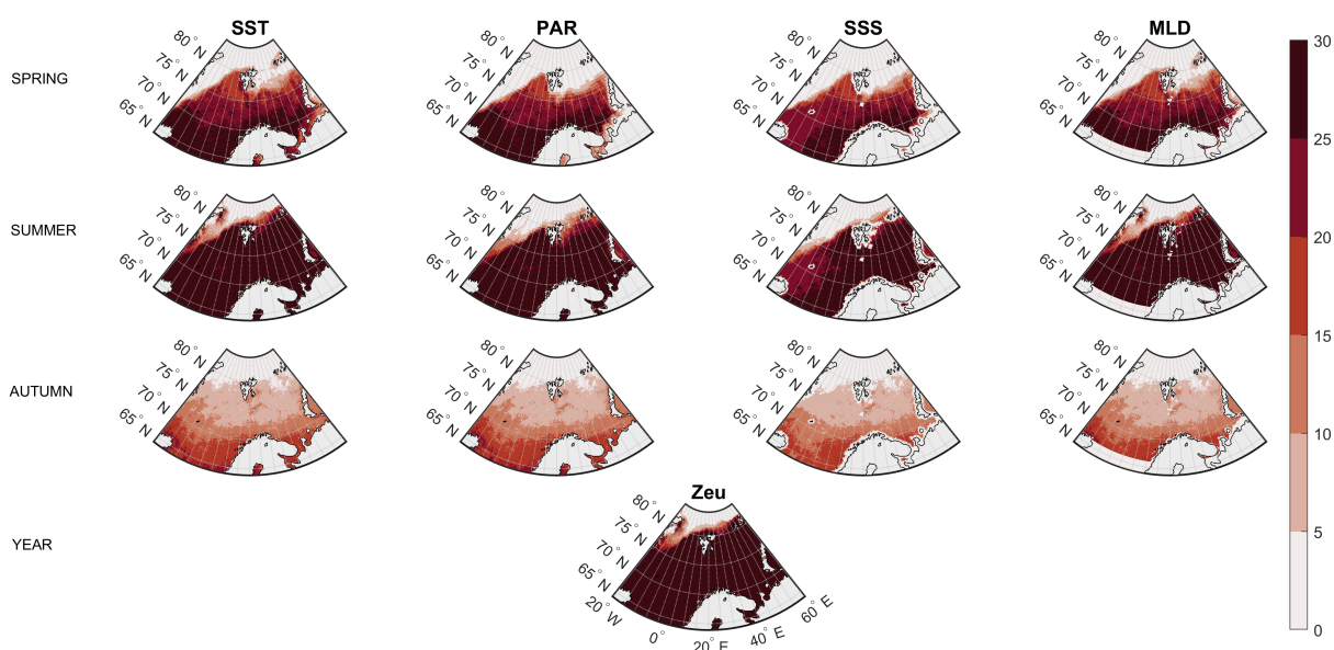
Figure A1. Size of dataset (N) used to calculate correlation coefficients between chlorophyll- a concentration (Chl- a , \text{mg m}^{-3} ) and environmental parameters: sea surface temperature (SST, ^{\circ}\text{C} ), photosynthetically active radiation (PAR, \text{E m}^{-2} \text{ day}^{-1} ), sea surface salinity (SSS, psu), mixed layer depth (MLD, m) and euphotic layer depth (Zeus, m) in 2010–2019.
