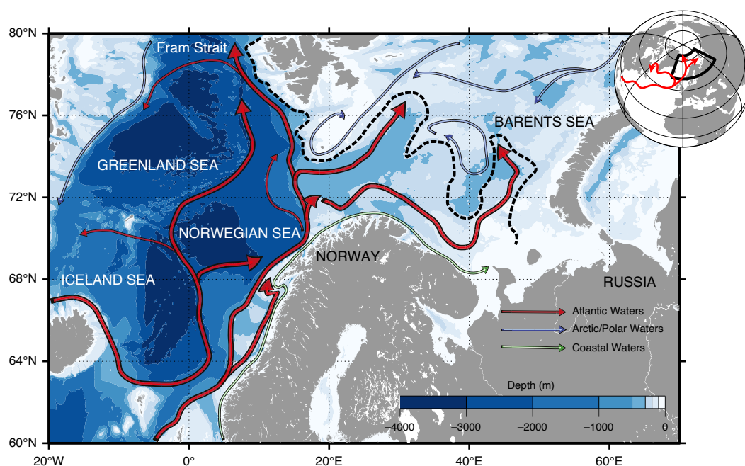
Figure 1. Map of the European Arctic Corridor. Surface currents are: polar waters in blue, coastal waters in green, Atlantic waters – in red. Dashed black line is the Barents Sea polar front. From [Oziel et al., 2020].
