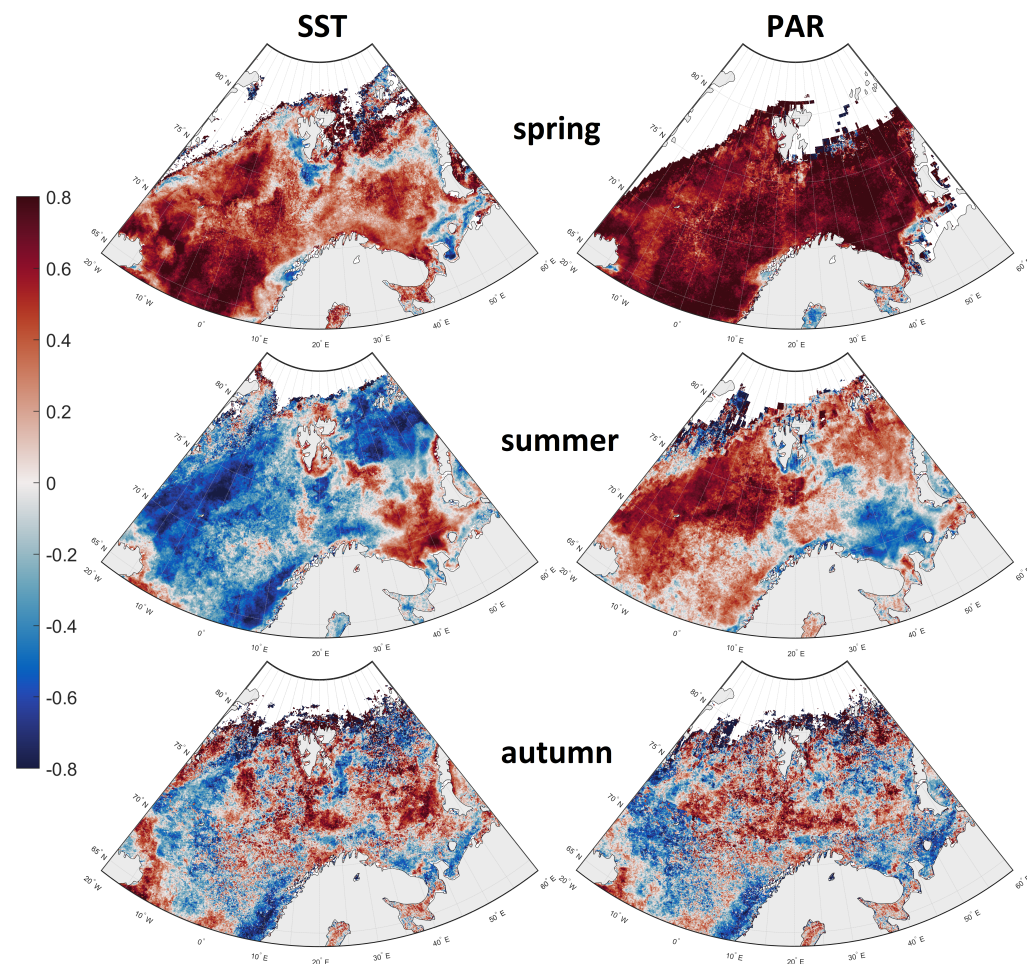
Figure 2. Spatial and temporal variability of a correlation coefficient between chlorophyll- a concentration (Chl- a , \text{mg m}^{-3} ) and environmental parameters: sea surface temperature (SST, ^{\circ}\text{C} ), and photosynthetically active radiation (PAR, \text{E m}^{-2} \text{ day}^{-1} ) in 2010–2019. The correlation coefficient is grouped and calculated by seasons. All correlation coefficients have a p -value \leq 0.05 .
