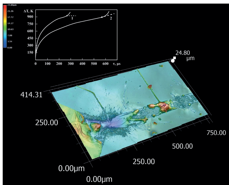
Fig. 8. Topography of the Al-Ti-Si structure after an electric explosion (current pulse amplitude j=13 \cdot 10^{10} A/m 2 and duration 600 \mu s). In the insert: The dynamics of the temperature of aluminum metallization \Delta T_i(t) = T_i(t) - T_0 during the passage of a single current pulse amplitude: 1 – j=8.7 \cdot 10^{10} A/m 2 ; 2 – 7.0 \cdot 10^{10} A/m 2 .
