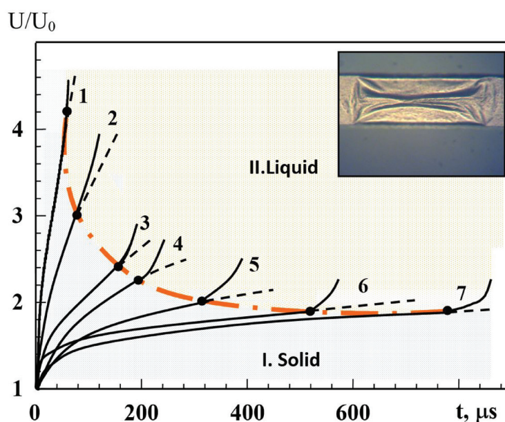
Fig. 2. The area of safe operation of the Al-Si contact (I. Solid zone) when passing through the structure of a single rectangular current pulse with an amplitude of: 1 – j=8.8 \cdot 10^{10} A/m 2 ; 2 – 8.6 \cdot 10^{10} A/m 2 ; 3 – 8.2 \cdot 10^{10} A/m 2 ; 4 – 6.7 \cdot 10^{10} A/m 2 ; 5 – 6.6 \cdot 10^{10} A/m 2 ; 6 – 6.1 \cdot 10^{10} A/m 2 ; 7 – 5.8 \cdot 10^{10} A/m 2 . Points 1–7 are the moment of oscillogram deviation associated with the beginning of contact melting processes at the Al-Si boundary and melting of the Al-film. In the insert: Microscopy of the structure at j=5.8 \cdot 10^{10} A/m 2 , pulse duration \tau=500 \mu s.
