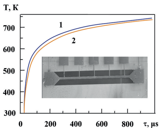
Fig. 9. Oscillograms of inclusion of metallization on silicon when passing a rectangular current pulse with an amplitude of j=7.1 \cdot 10^{10} A/m 2 and a duration of 950 \mu s: 1 – copper-based metallization system with carbon nanotubes; 2 – sample witness. On the insert: A photo of the test structure; the size of the contact pad is 100 × 100 \mu m.
