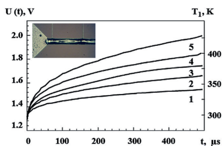
Fig. 6. Oscillograms of the Si-Ti-Al system activation at different thickness of the Ti sublayer: 1 – h_2 = 0 ; 2 – h_2 = 80 ; 3 – h_2 = 100 ; 4 – h_2 = 130 ; 5 – h_2 = 170\ \text{nm} ; j = 6.0 \cdot 10^{10}\ \text{A/m}^2 ; h_1 = 2\ \mu\text{m} ; duration pulses of 500\ \mu\text{s} . On the insert: Photo of the Al-Ti-Si structure after passing a current pulse j > j_{cr} .
