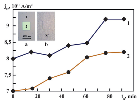
Fig. 7. The dependence of the value of the critical current density j_c on the annealing time of the t_h structure Al-Ti-Si in an inert atmosphere at a temperature of 500 °C; the duration of the rectangular current pulse: 1 – 550 \mu s; 2 – 200 \mu s. In the insert: Micrograph of a multilayer structure Al-(Ti,Ni)-Si: a – windows 2 opened in oxide 1 for spraying the sublayer and the main current-carrying layer; b – after spraying the contacts.
