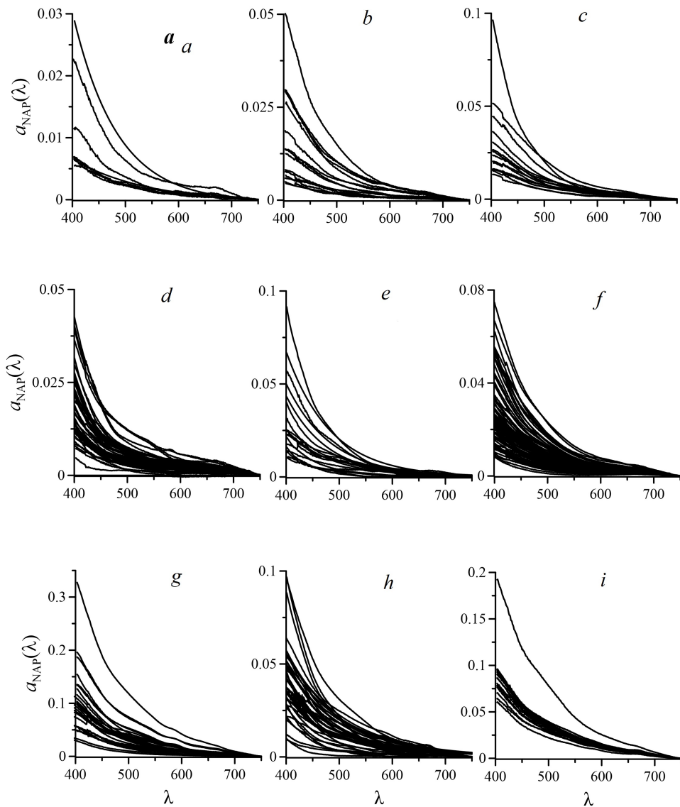
Fig. 3. Spectra of light absorption coefficients of non-algal particles ( a_{NAP}(\lambda) ) in the surface layers of the Arctic Ocean (a), the Barents (b) and Norwegian (c) seas, Atlantic sector of the Southern Ocean (d), the Black Sea in winter (e) and summer (f), the Sea of Azov (g), and the Baikal (h) and Teletskoye (i) lakes
