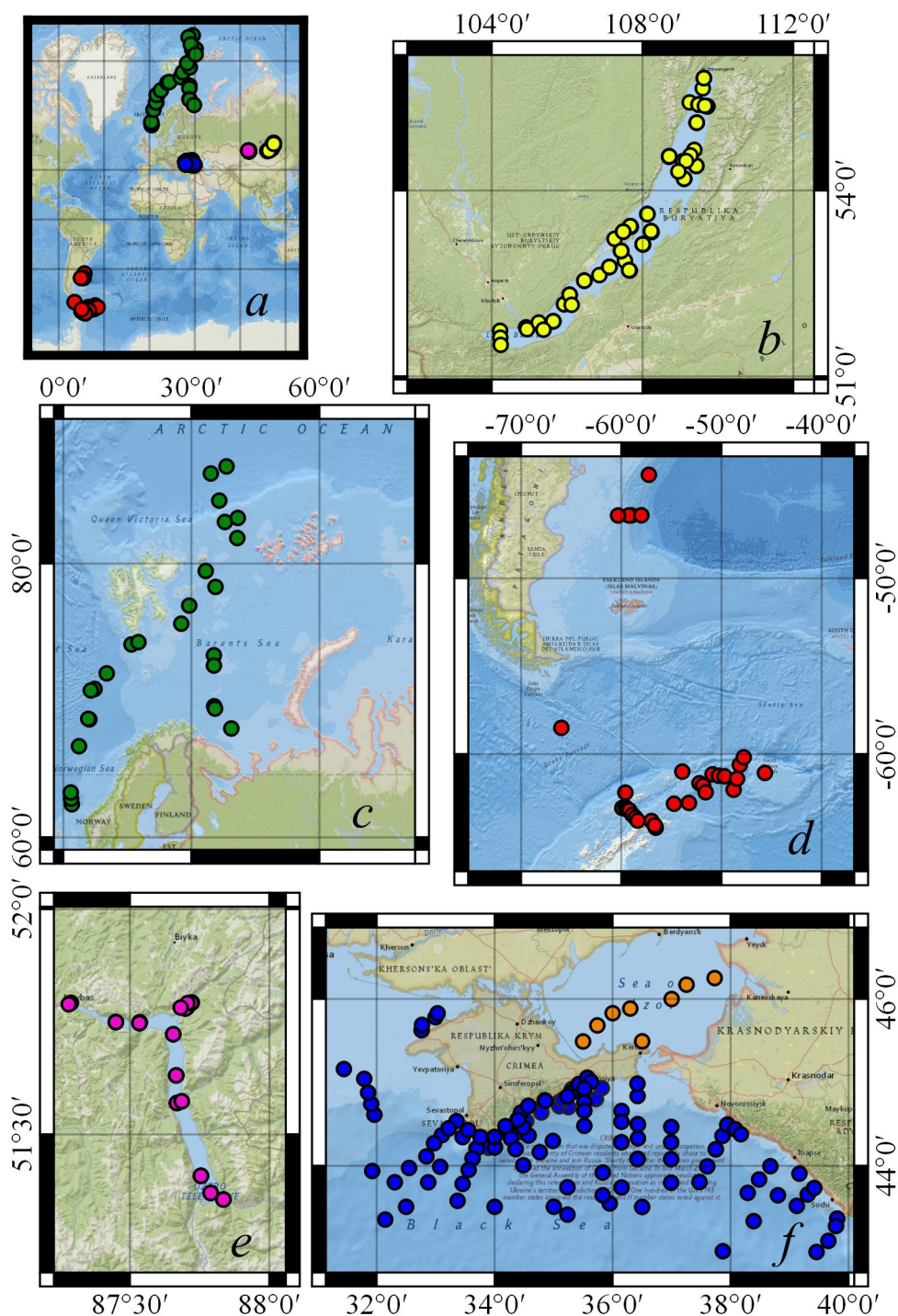
Fig. 1. Location of stations (marked with colored circles) in the study areas of the World Ocean ( a ); enlarged image of the study areas: b – Lake Baikal (yellow), c – Barents and Norwegian seas, and Arctic Ocean (green), d – Atlantic sector of the Southern Ocean (red), e – Lake Teletskoye (purple), f – Black (blue) and Azov (brown) seas
