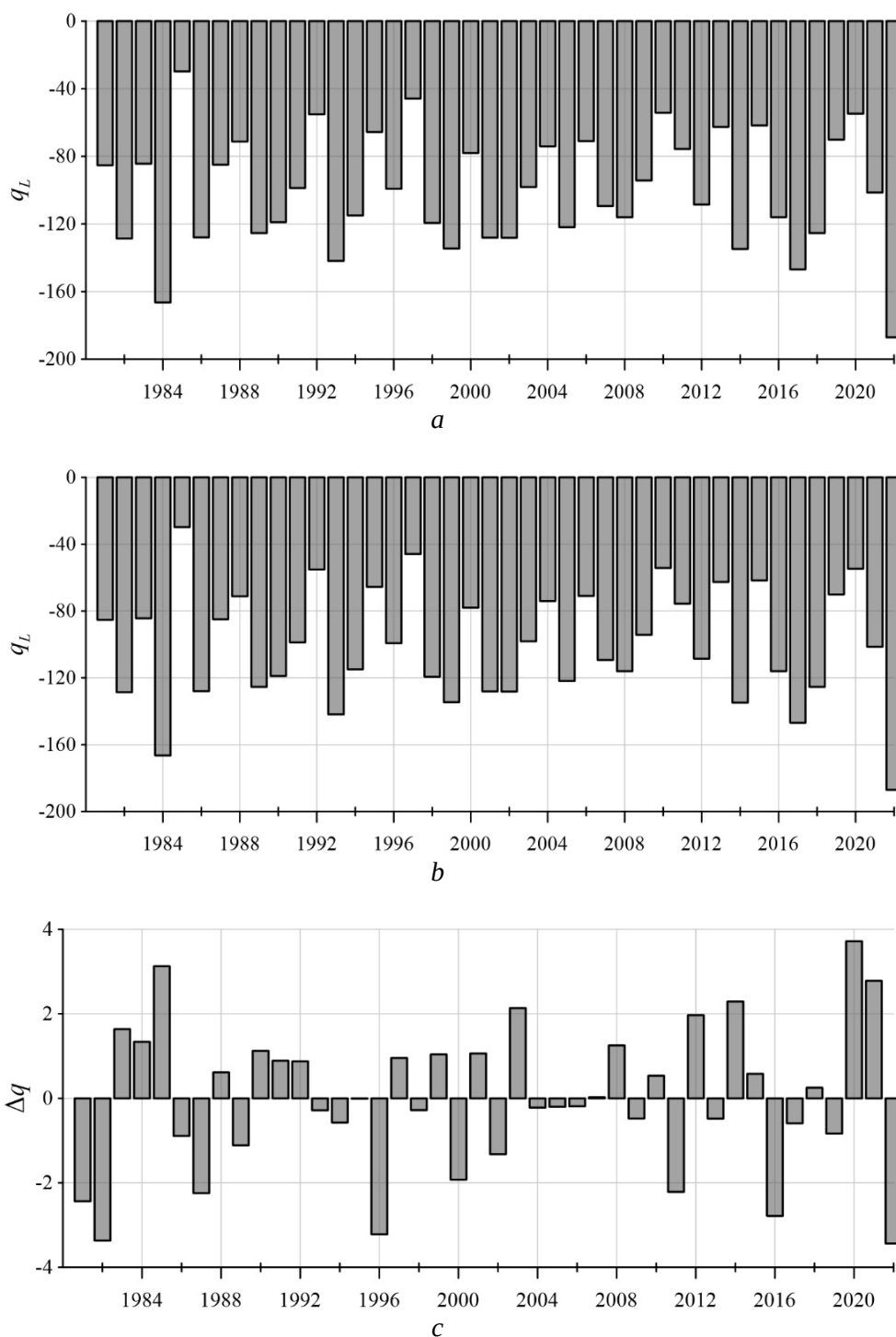
Fig. 16. Mean annual values of sediment rates: a – at the southeastern boundary ( x = 0 ); b – at the northwestern boundary ( x = L ); c – difference between the sediment rates at the southeastern and northwestern boundaries
