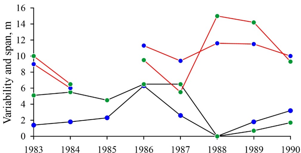
Fig. 2. Interannual variability of the coastline position (black curves) and the range of its seasonal fluctuations (red curves). Blue points show the western part of the Lake Sasyk bay-bar, green ones – its eastern part
