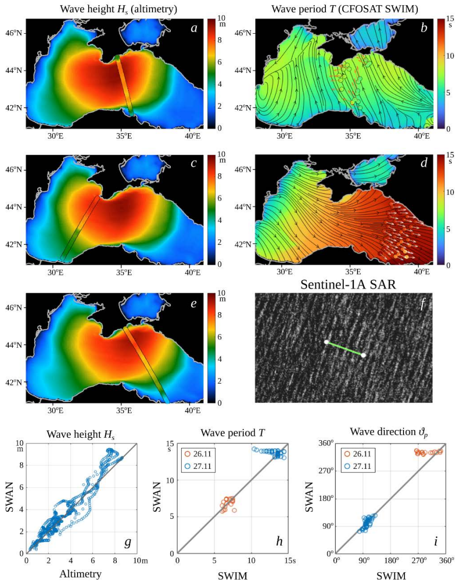
F i g. 6. Comparison of model calculations and satellite data: simulated wave height fields with the superimposed altimeter data from 26 November at 19:06 (a), 20:23 (c), 21:46 (e); simulated fields of wave periods and directions with the superimposed SWIM data from 26 November at 04:49 (b) and 27 November at 04:35 (d); fragment of SAR image with the superimposed line of 1 km long (f). Comparison of simulations and satellite data in terms of wave heights (g), periods (h) and directions (i)
